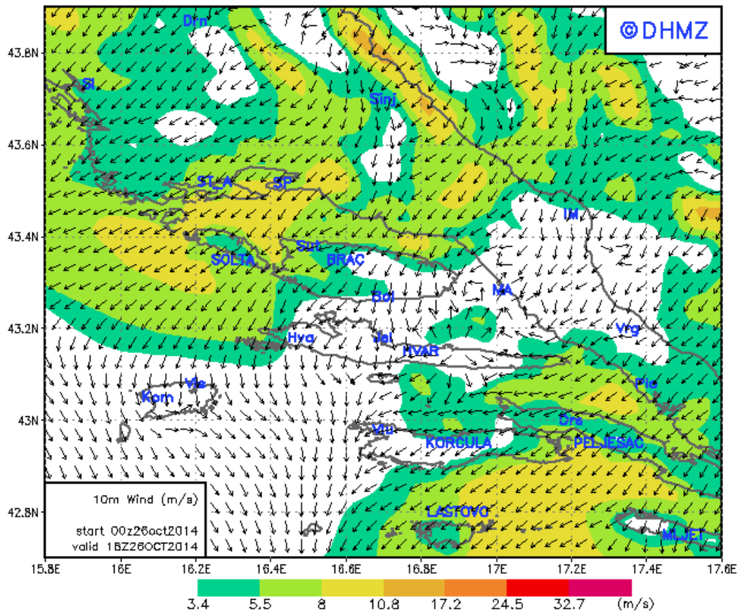
DADA Split 10m Wind at 18 UTC 26OCT2014
