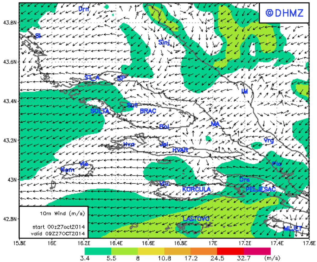
DAdA Split 10m Wind at 09 UTC 27OCT2014
