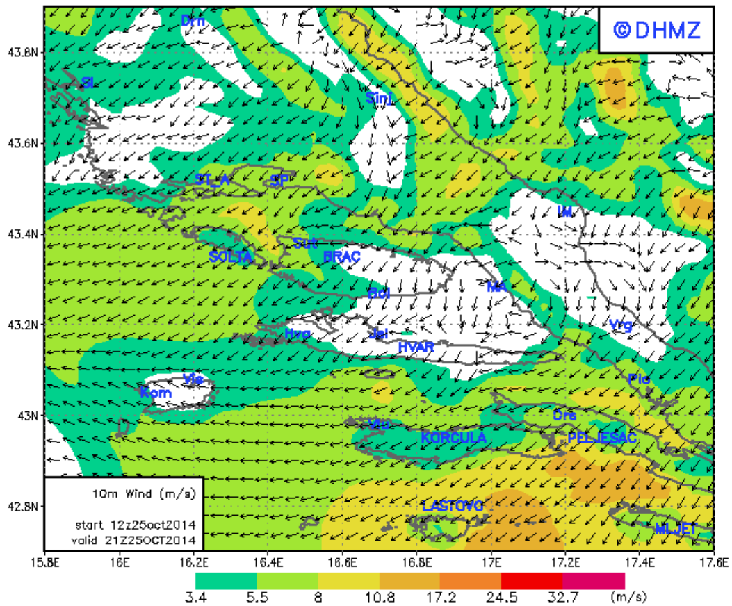
DAdA Split 10m Wind at 21 UTC 25OCT2014
