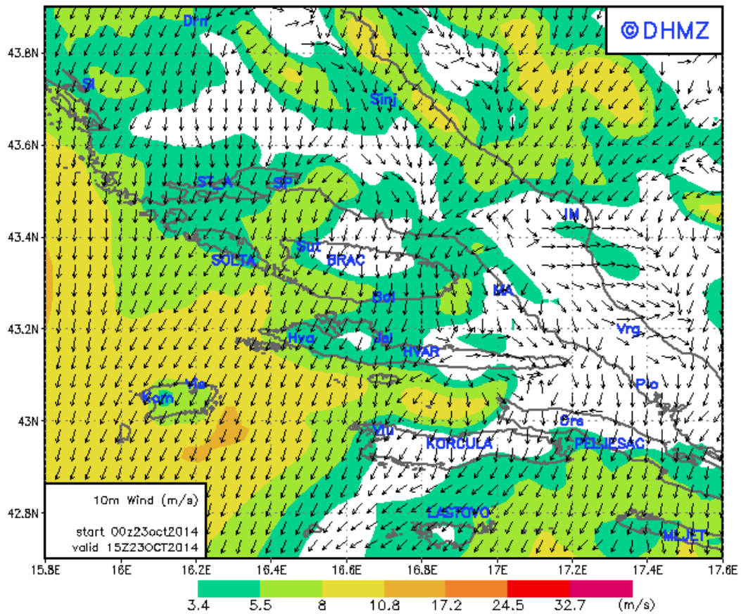
DAdA Split 10m Wind at 15 UTC 23OCT2014
