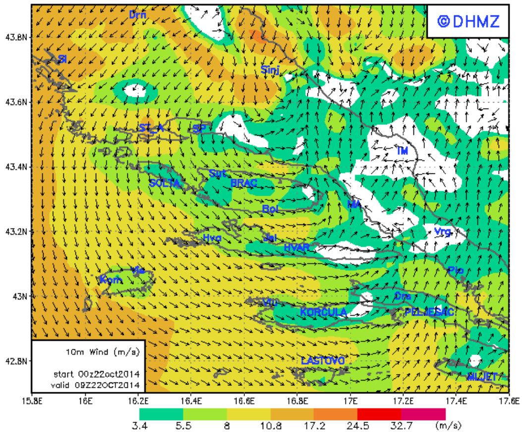
DAdA Split 10m Wind at 09 UTC 22OCT2014
