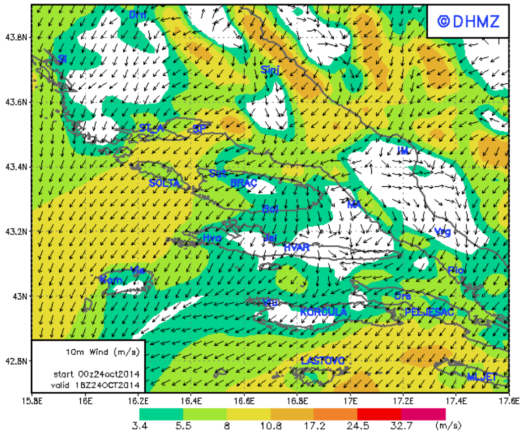
DAdA Split 10m Wind at 18 UTC 24OCT2014
