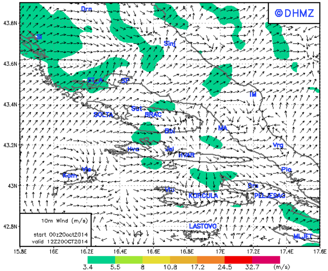
DAdA Split 10m Wind at 12 UTC 20OCT2014
