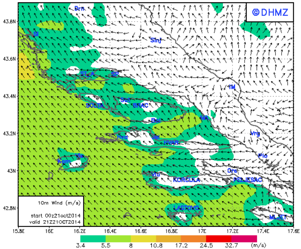
DAdA Split 10m Wind at 21 UTC 21OCT2014
