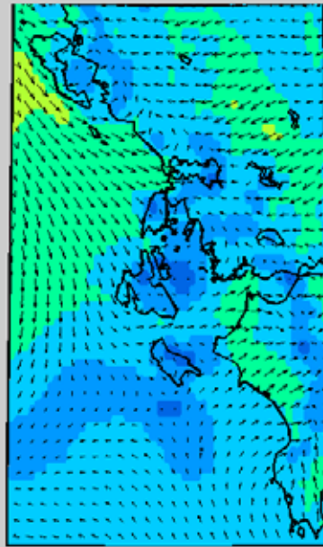
Ionian sea Surface wind (10m) on Thursday (13/08/15) 12:00UTC
