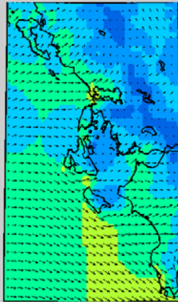
Ionian sea Surface wind (10m) on Monday (10/08/15) 12:00UTC
