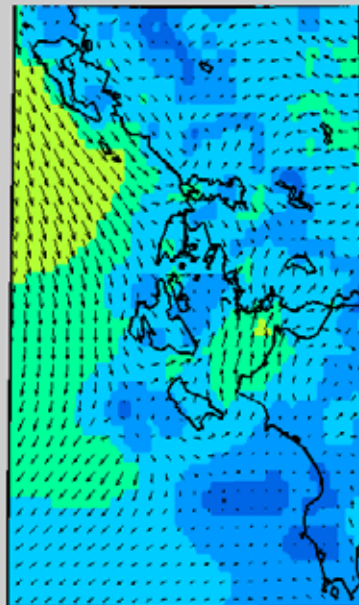
Ionian sea Surface wind (10m) on Thursday (13/08/15) 18:00UTC
