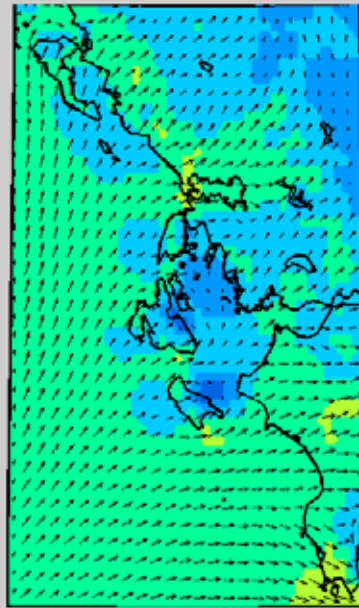
Ionian sea Surface wind (10m) on Tuesday (11/08/15) 12:00UTC
