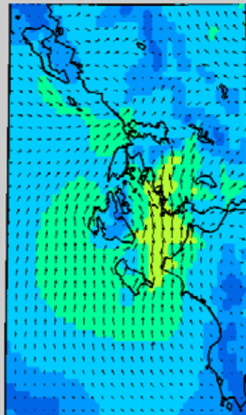
Ionian sea Surface wind (10m) on Friday (14/08/15) 18:00UTC
