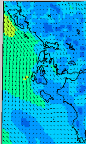
Ionian sea Surface wind (10m) on Wednesday (12/08/15) 18:00UTC
