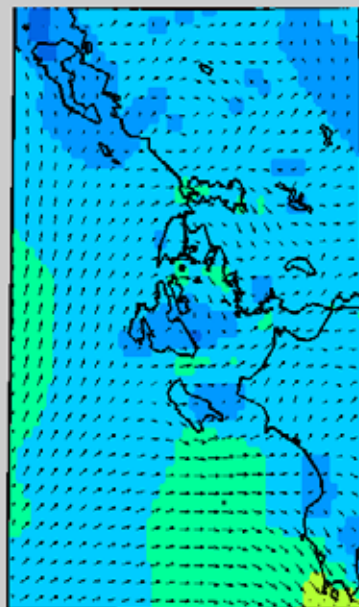
Ionian sea Surface wind (10m) on Tuesday (11/08/15) 18:00UTC
