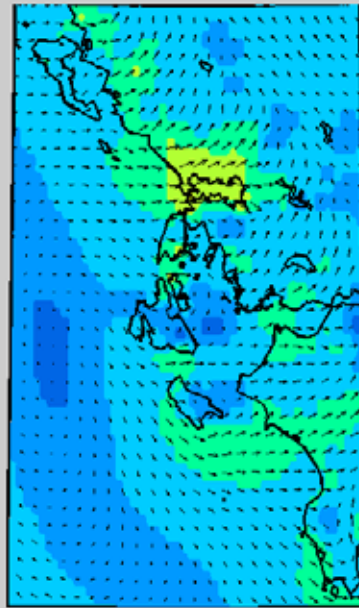
Ionian sea Surface wind (10m) on Wednesday (12/08/15) 12:00UTC
