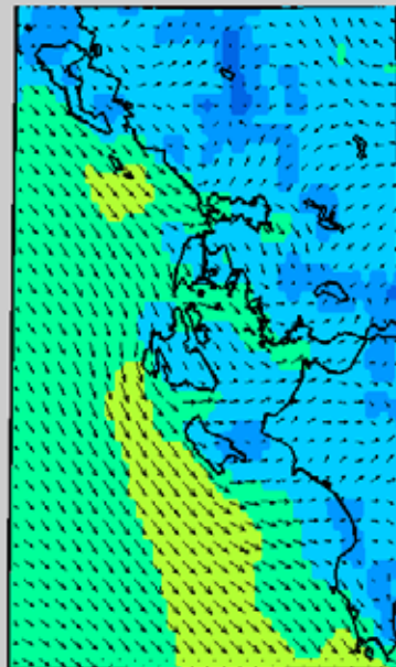
Ionian sea Surface wind (10m) on Sunday (09/08/15) 18:00UTC
