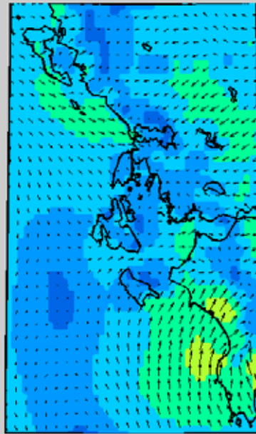
Ionian sea Surface wind (10m) on Friday (14/08/15) 12:00UTC
