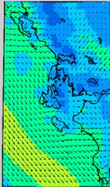
Ionian sea Surface wind (10m) on Sunday (09/08/15) 12:00UTC
