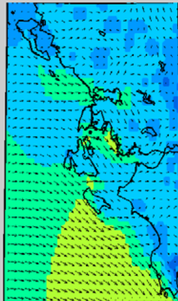
Ionian sea Surface wind (10m) on Monday (10/08/15) 18:00UTC
