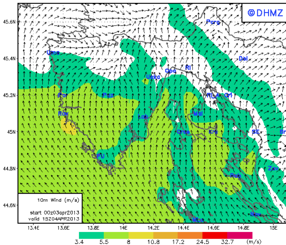
DAdA Senj 10m Wind on 15 UTC 04APR2013
