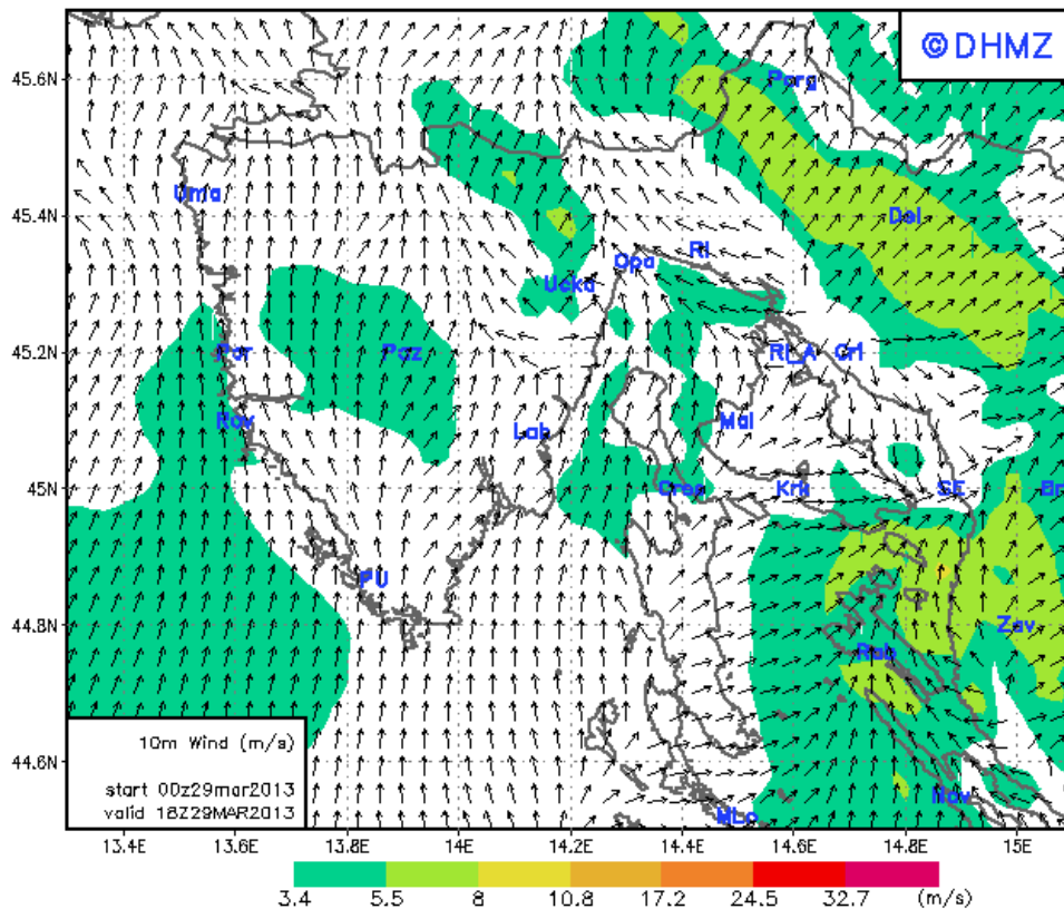
DAda Senj 10m Wind on 18 UTC 29MAR2013
